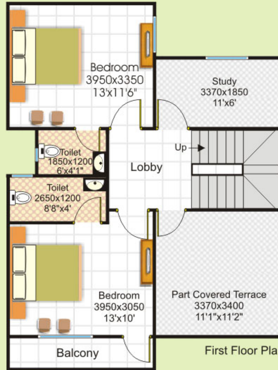
Plot Size - 7.62x12.20 25'x40' (3 BHK) Super built up area : 1555.70 Sq. Ft.
